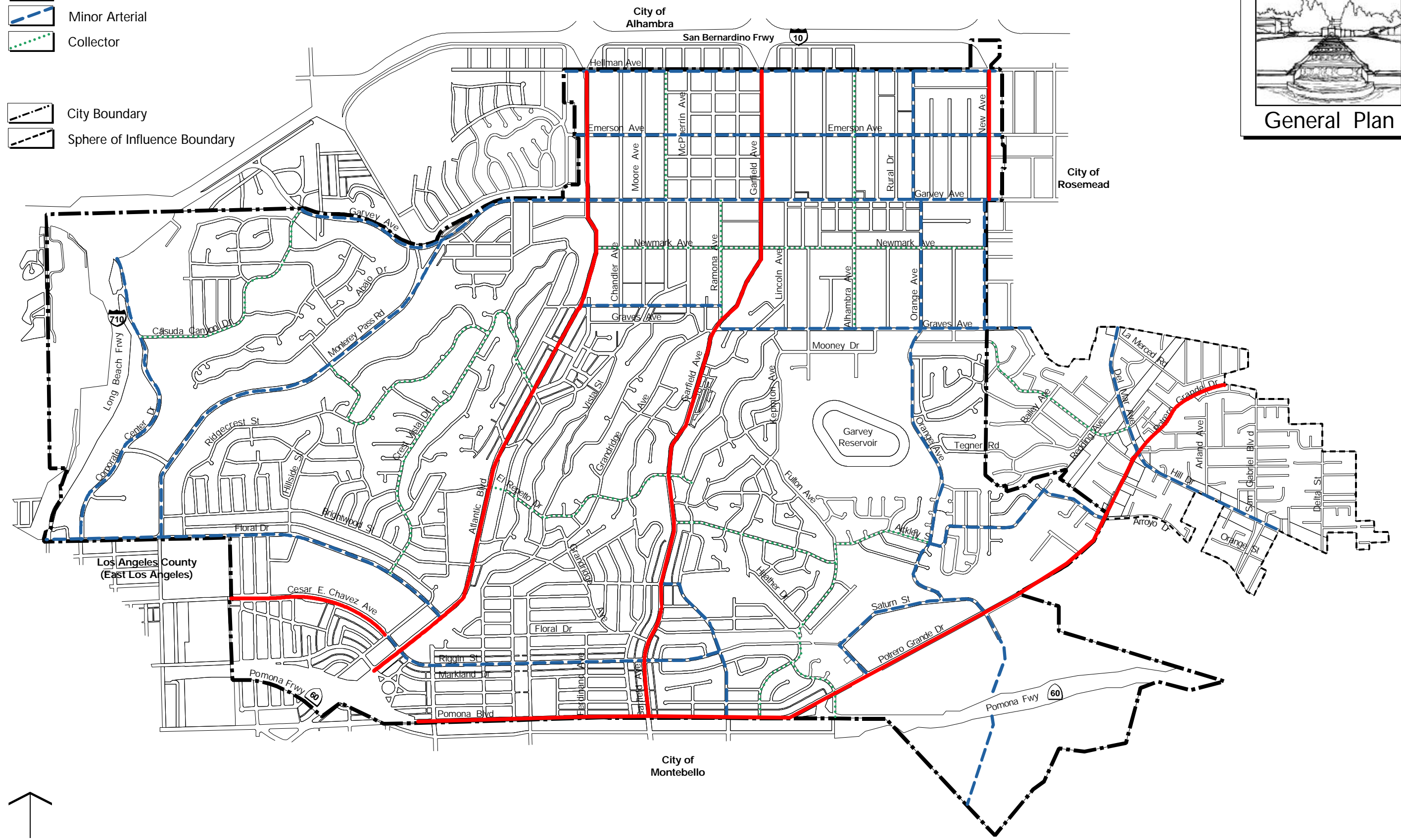
Figure C-2 Master Circulation Plan
